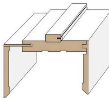
Double Rabbet Half Telescopic Jamb with Rubber Seal, L-Shaped Casing on One Side and Flat Casing on the Other Side. Extension is Optional.
