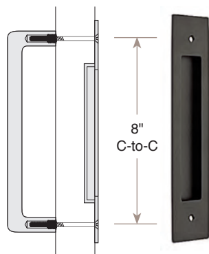
Modern Rectangular Flush Pull (Flush Pull Only) Drilled to accept 8" pull
